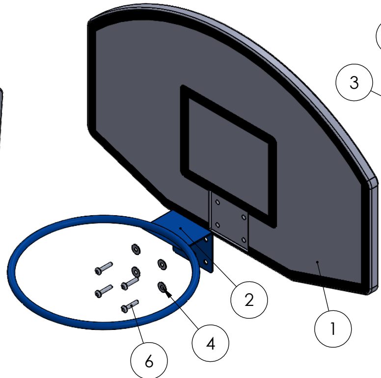
EXPLODED VIEW
