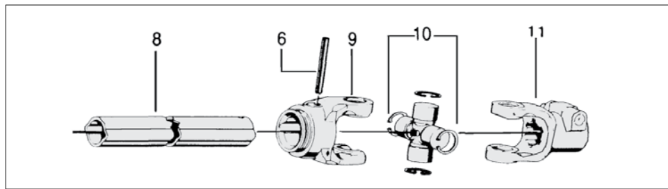
A. WWE IMPLEMENT HALF (STANDARD JOINT).
