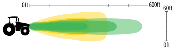
Part No. LB52300 COMBO FLOOD/SPOT LIGHT BAR - 52"
