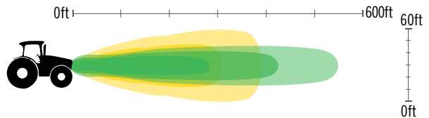
Part No. LB50288 COMBO FLOOD/SPOT LIGHT BAR - 50"
