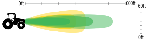
Part No. LB42240 COMBO FLOOD/SPOT LIGHT BAR - 42"
