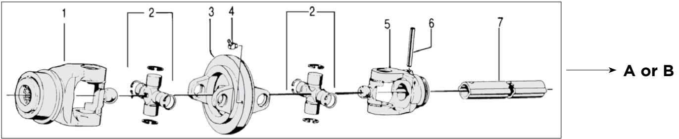
A. WWE IMPLEMENT HALF (STANDARD JOINT).
