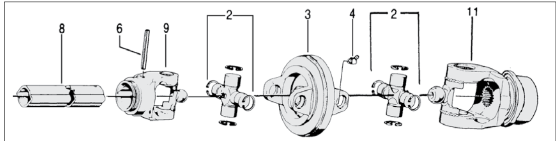
B. WWZ, TRACTOR END + IMPLEMENTS END CV
