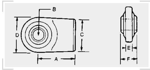
BENT LIFT ARM END
