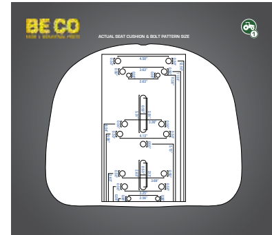
ACTUAL SIZE SEAT CUSHION & DETAILED BOLT PATTERN ON THE LID OF THE BOX
