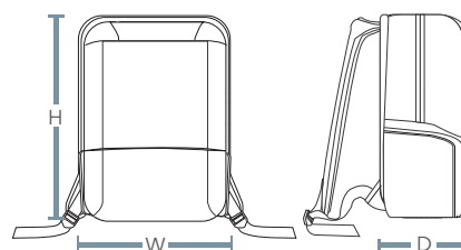
Overall dimensions.
