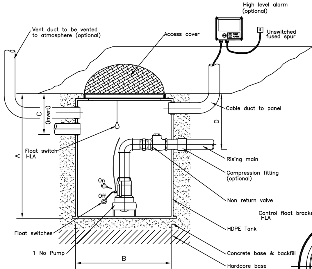
SIDE ELEVATION
