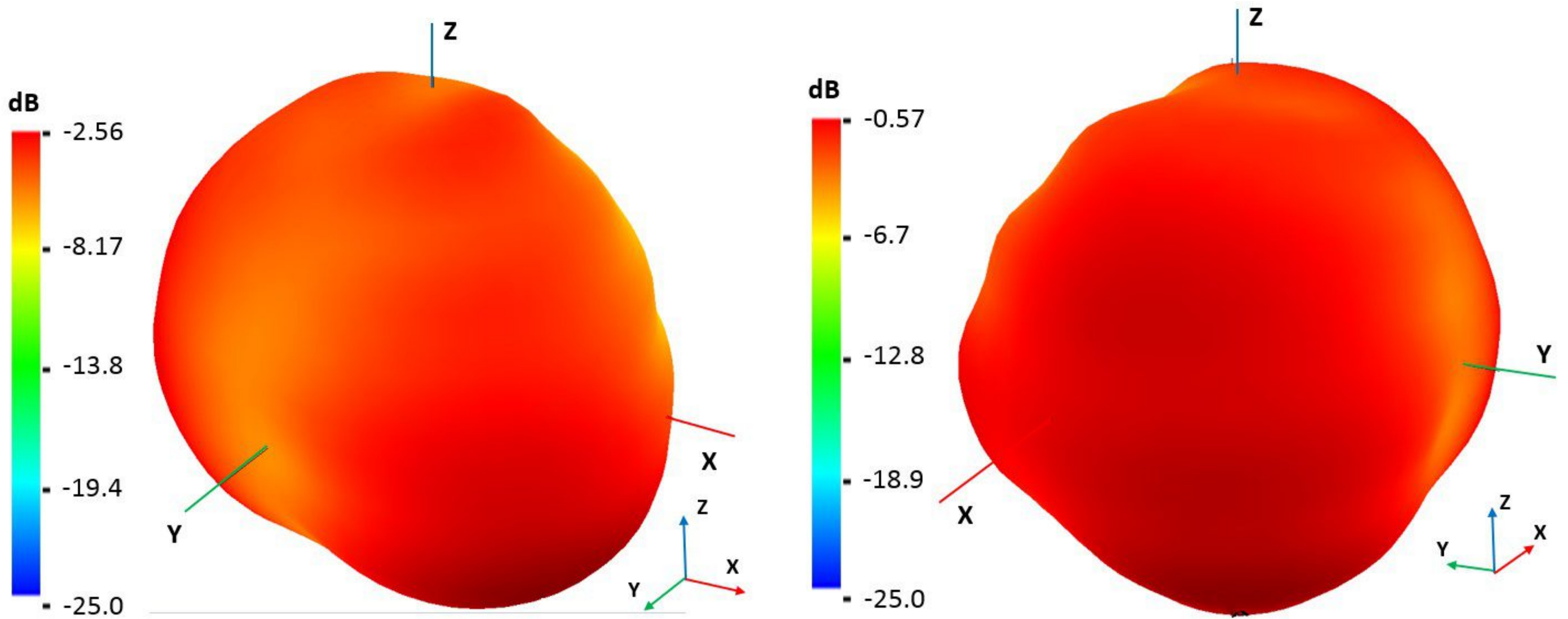
850 and 940 MHz Radiation pattern
