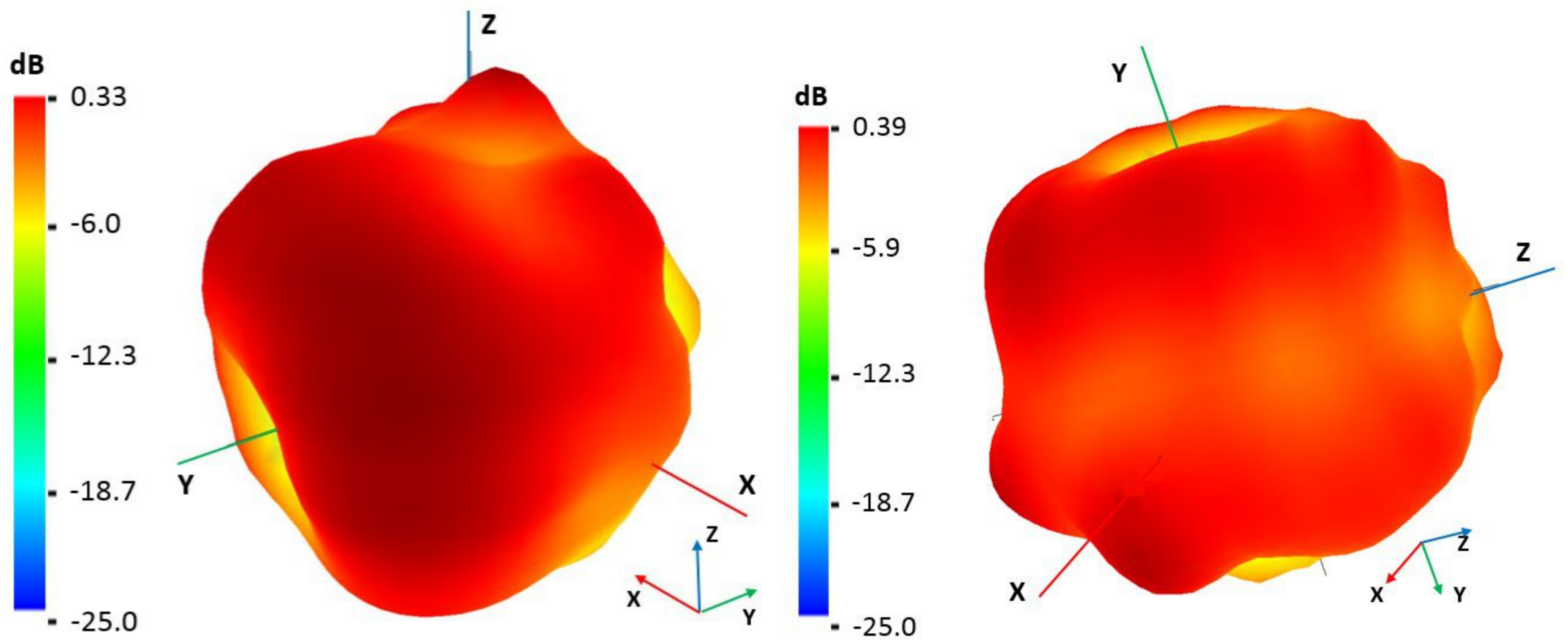
1750 and 1850 MHz Radiation pattern
