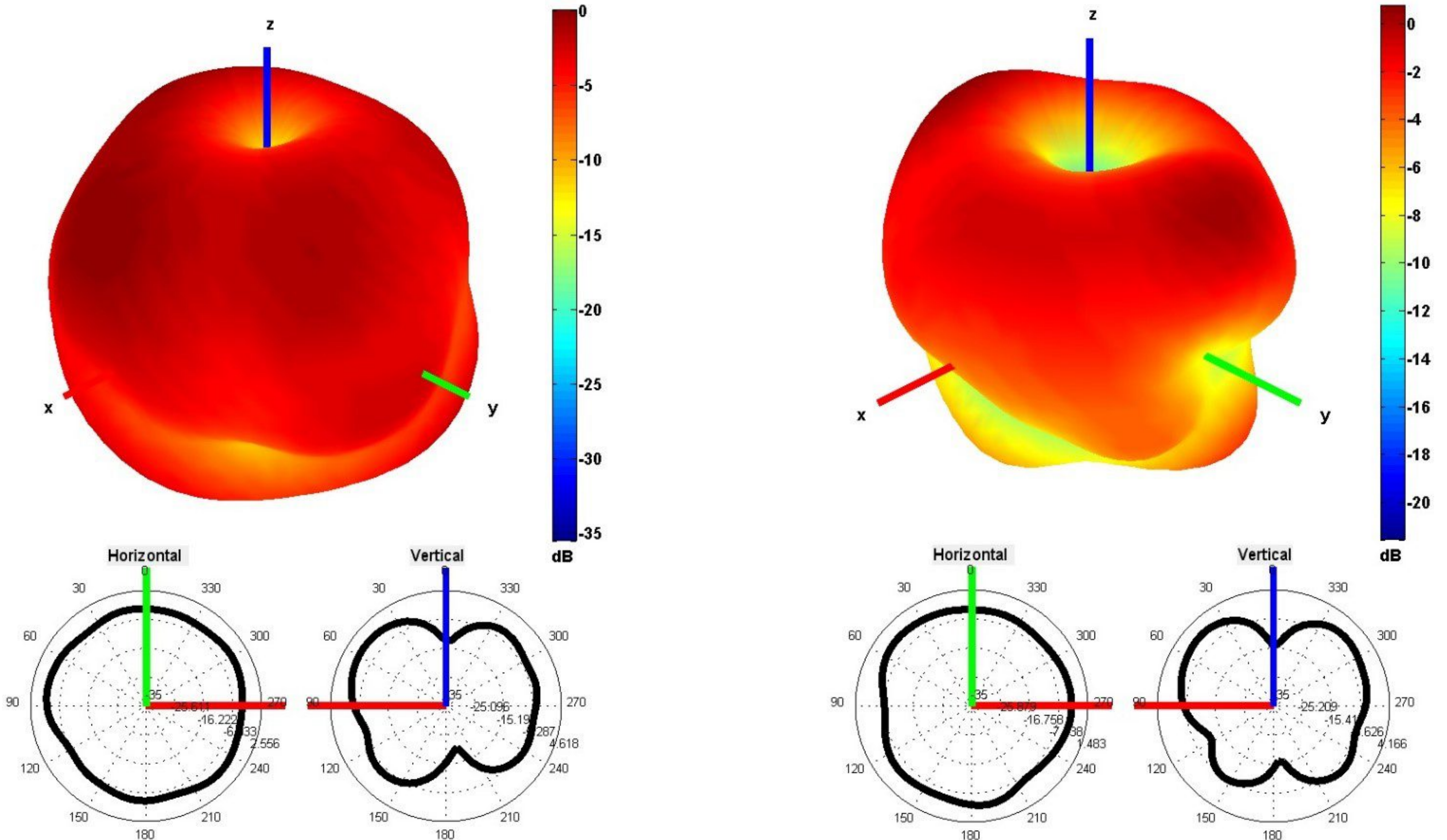
Cable 2: CELLULAR/LTE
