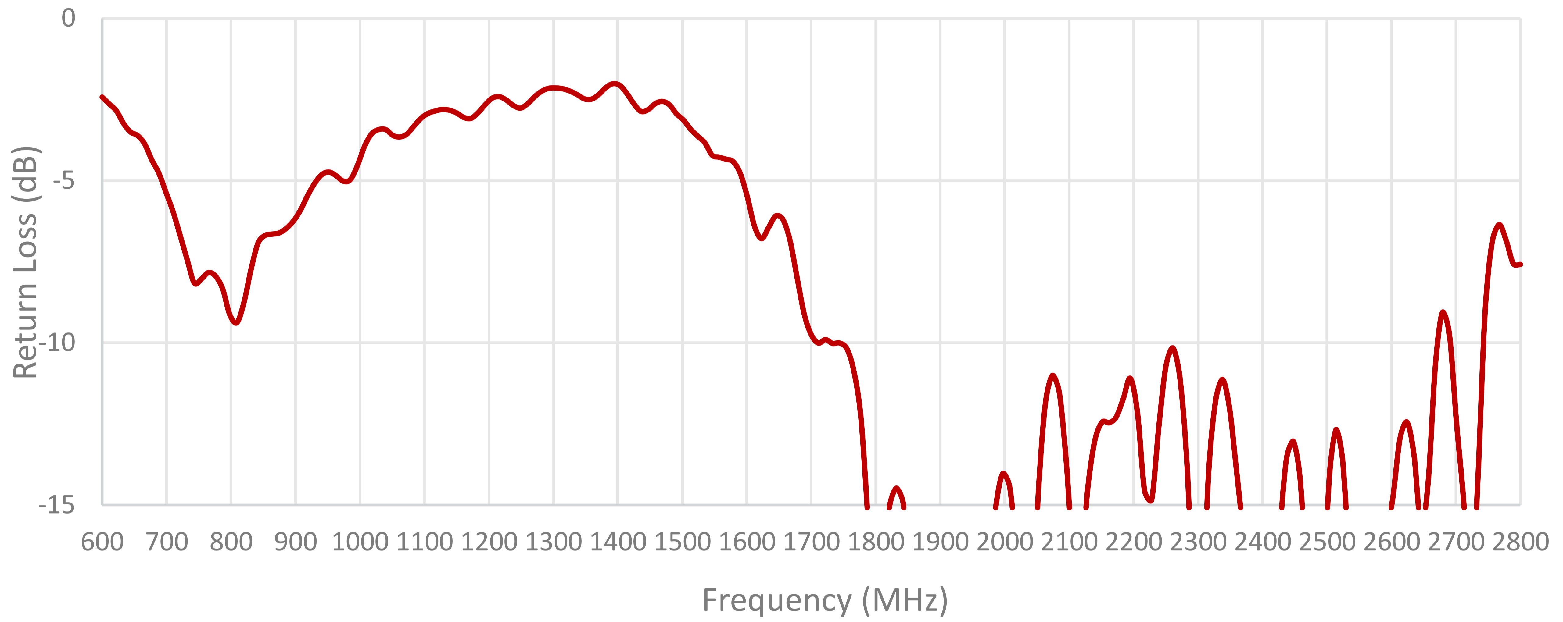
Cable 2: CELLULAR/LTE
