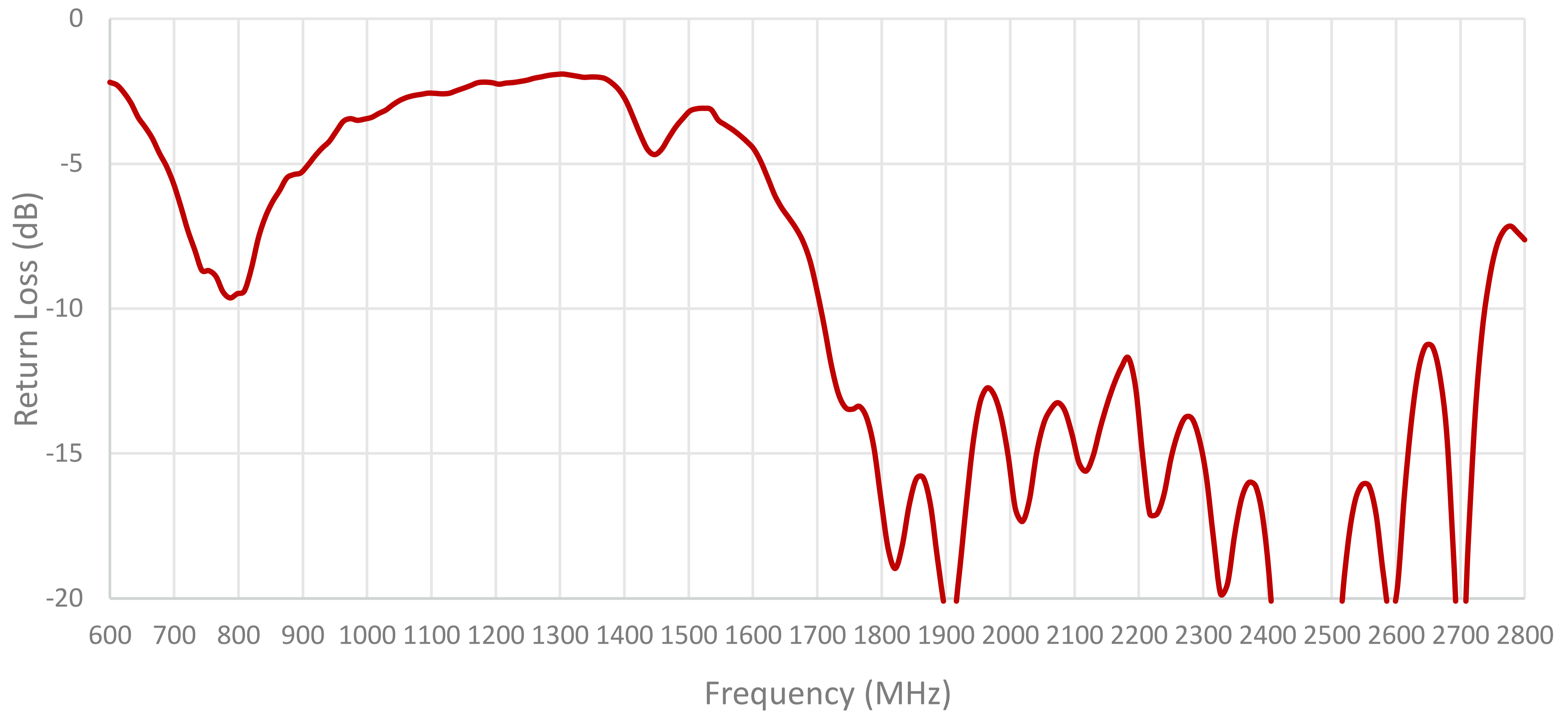
Cable 1: CELLULAR/LTE
