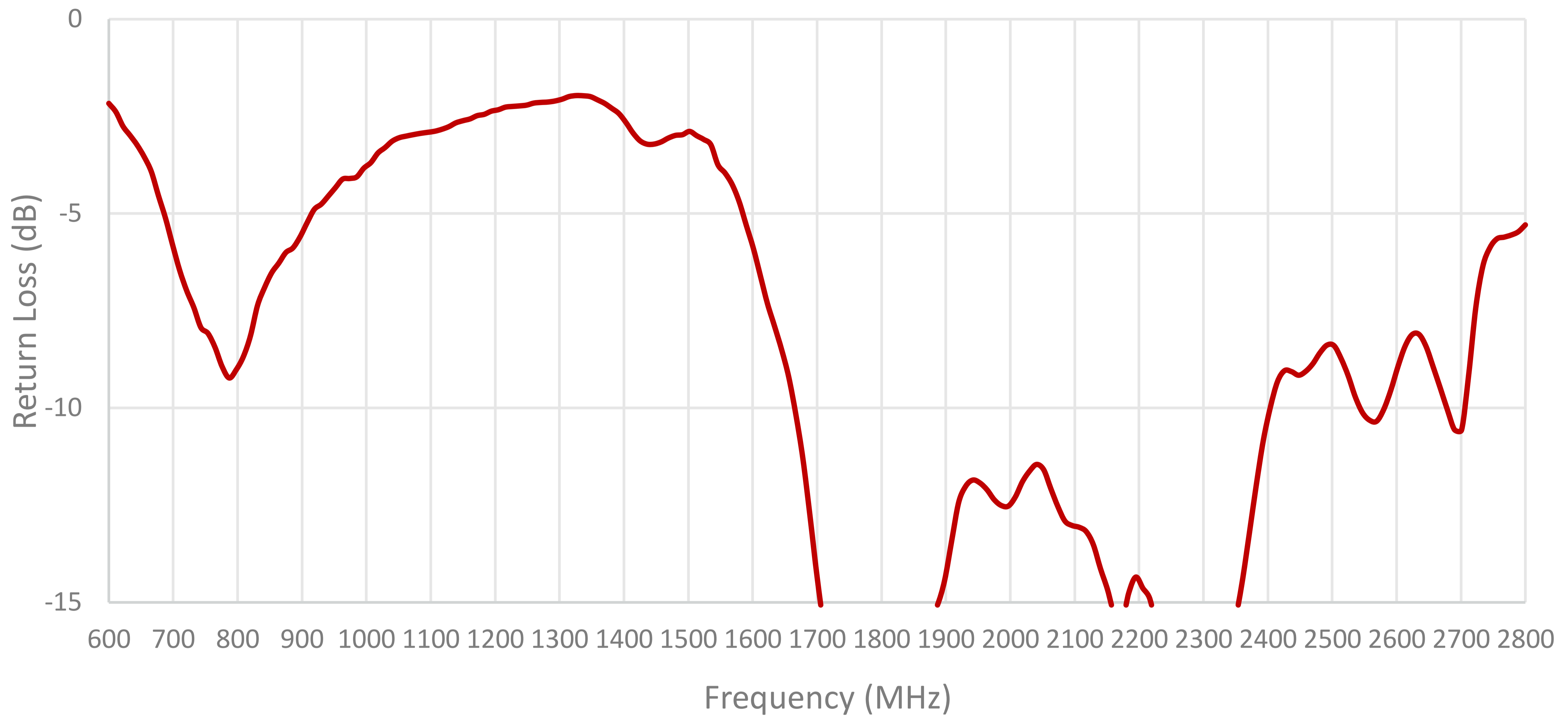
Cable 2: CELLULAR/LTE
