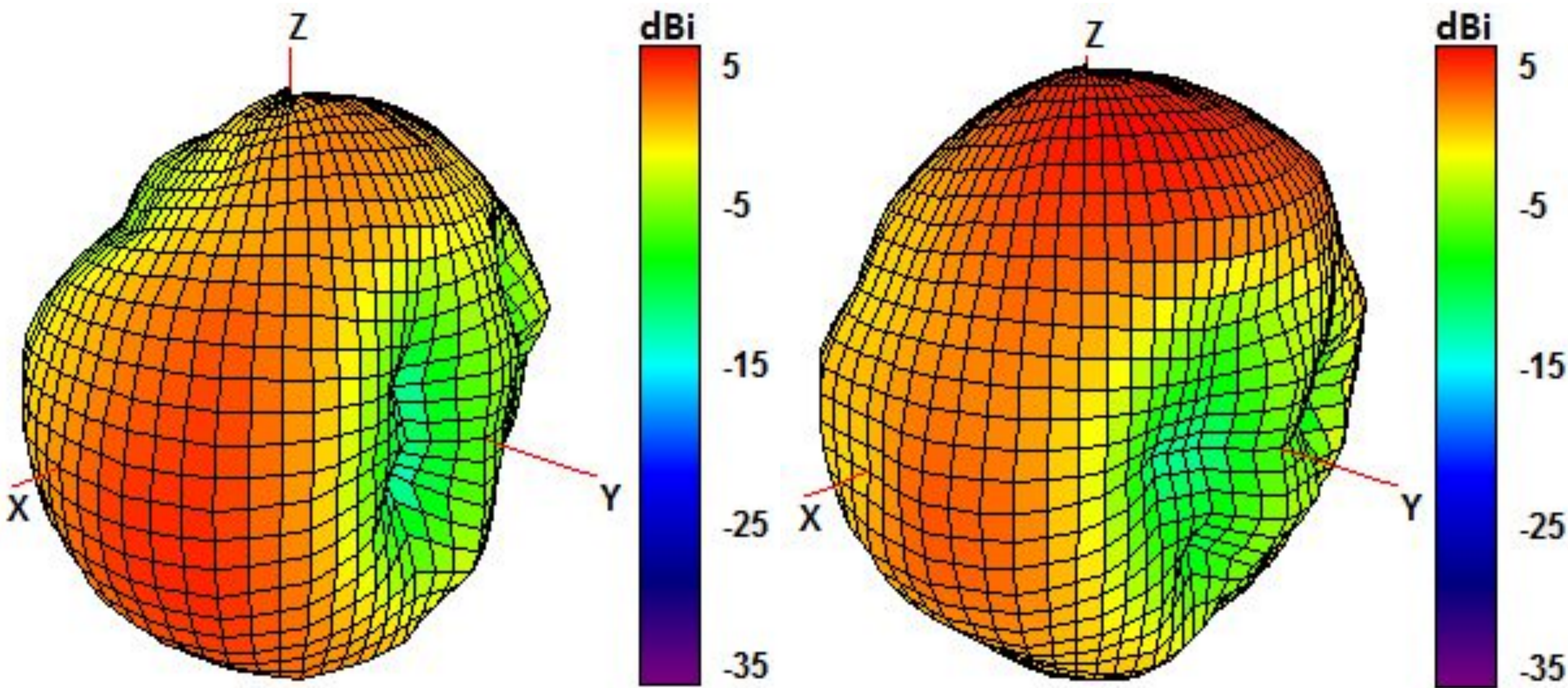
1850 and 1950 MHz Radiation pattern
