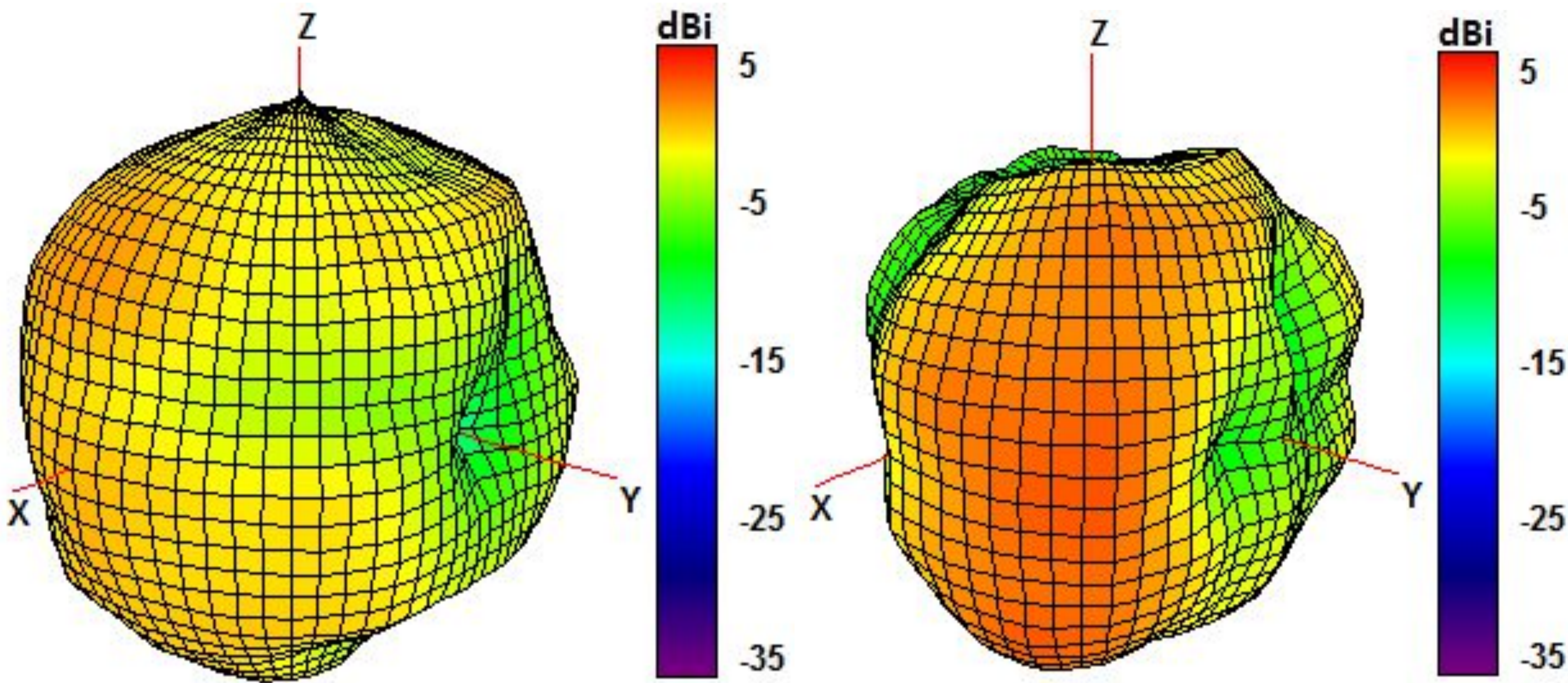
940 and 1750 MHz Radiation pattern
