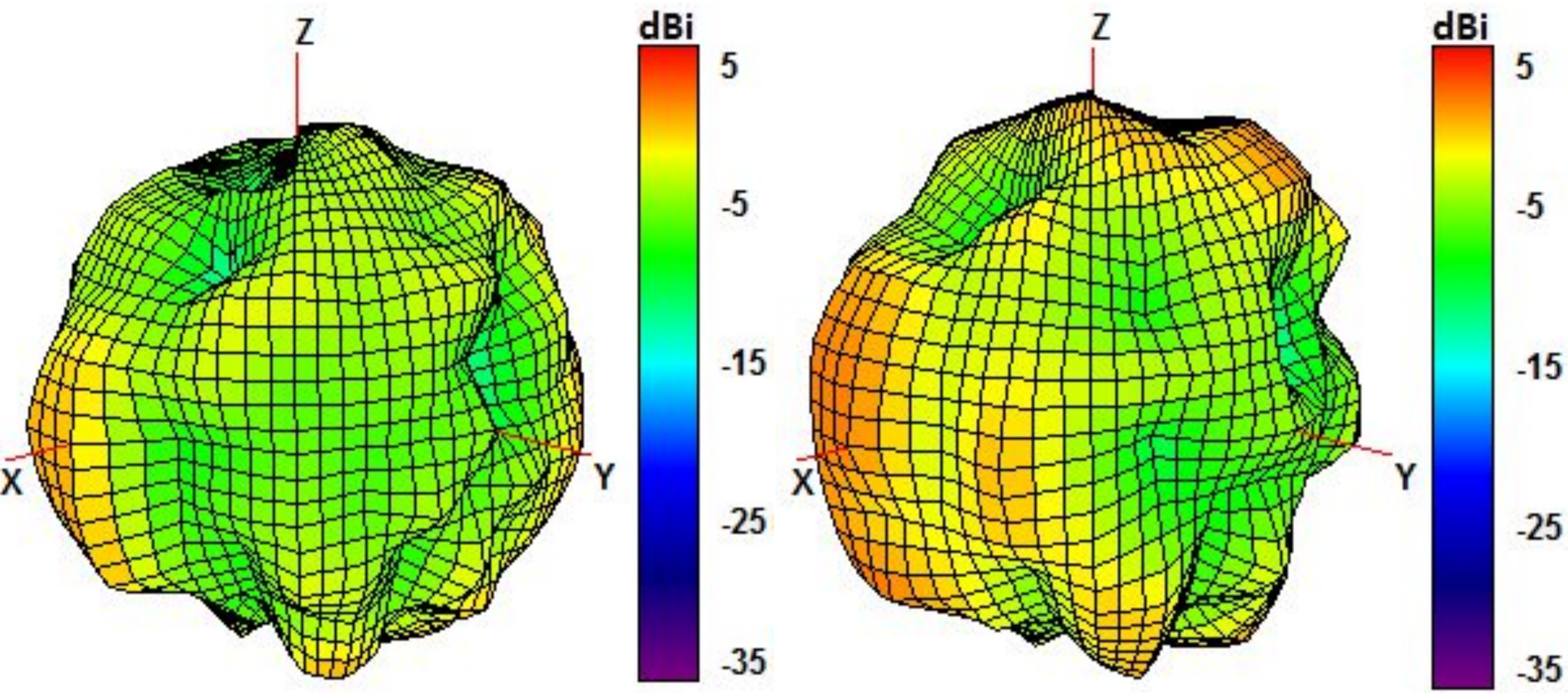
1850 and 1950 MHz Radiation pattern
