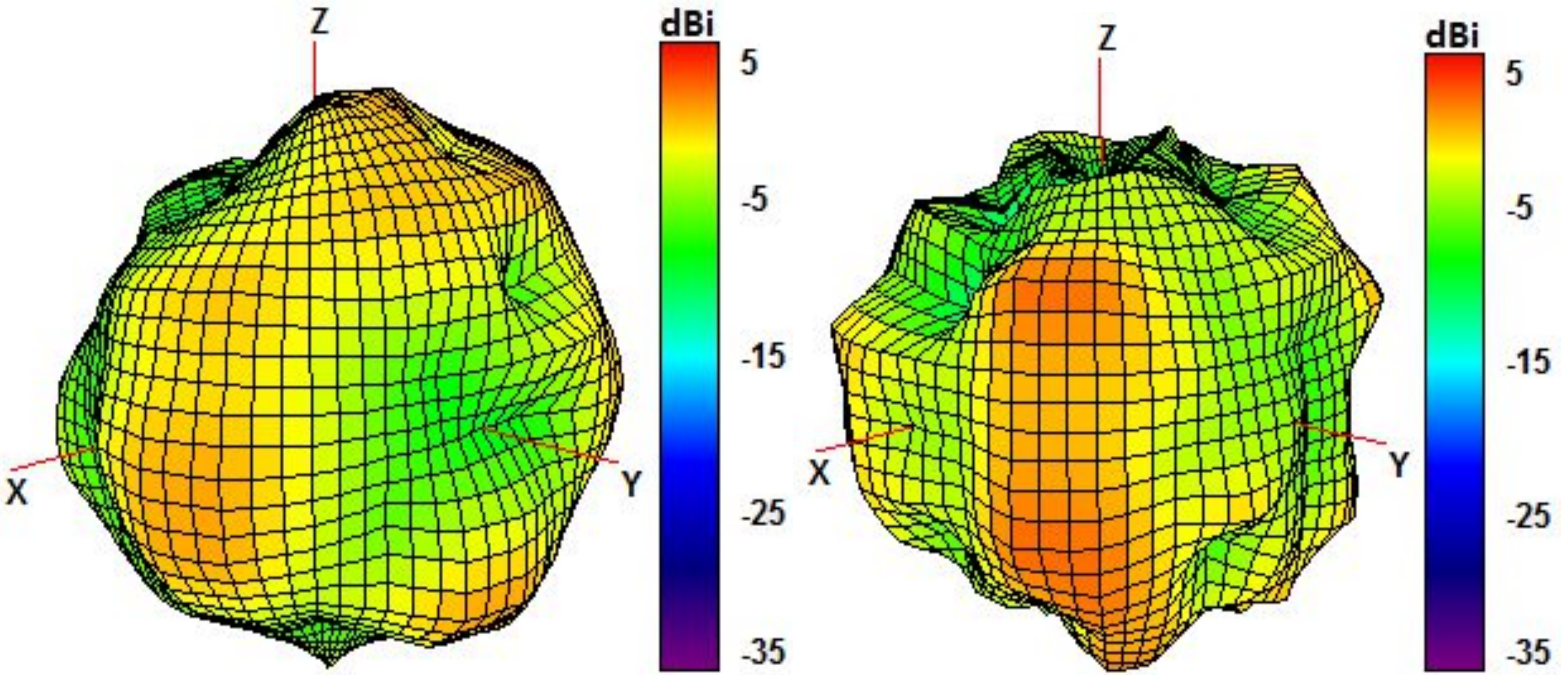
940 and 1750 MHz Radiation pattern
