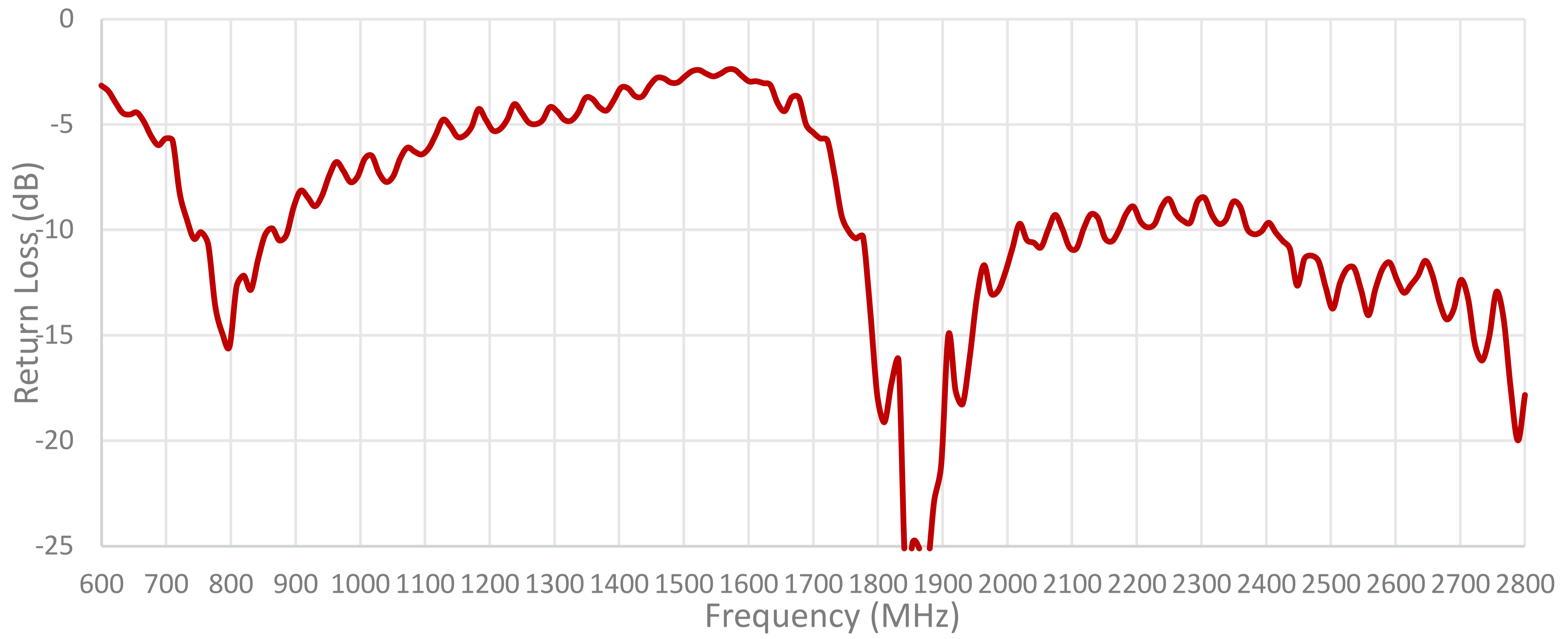
Cable 2: CELLULAR/LTE
