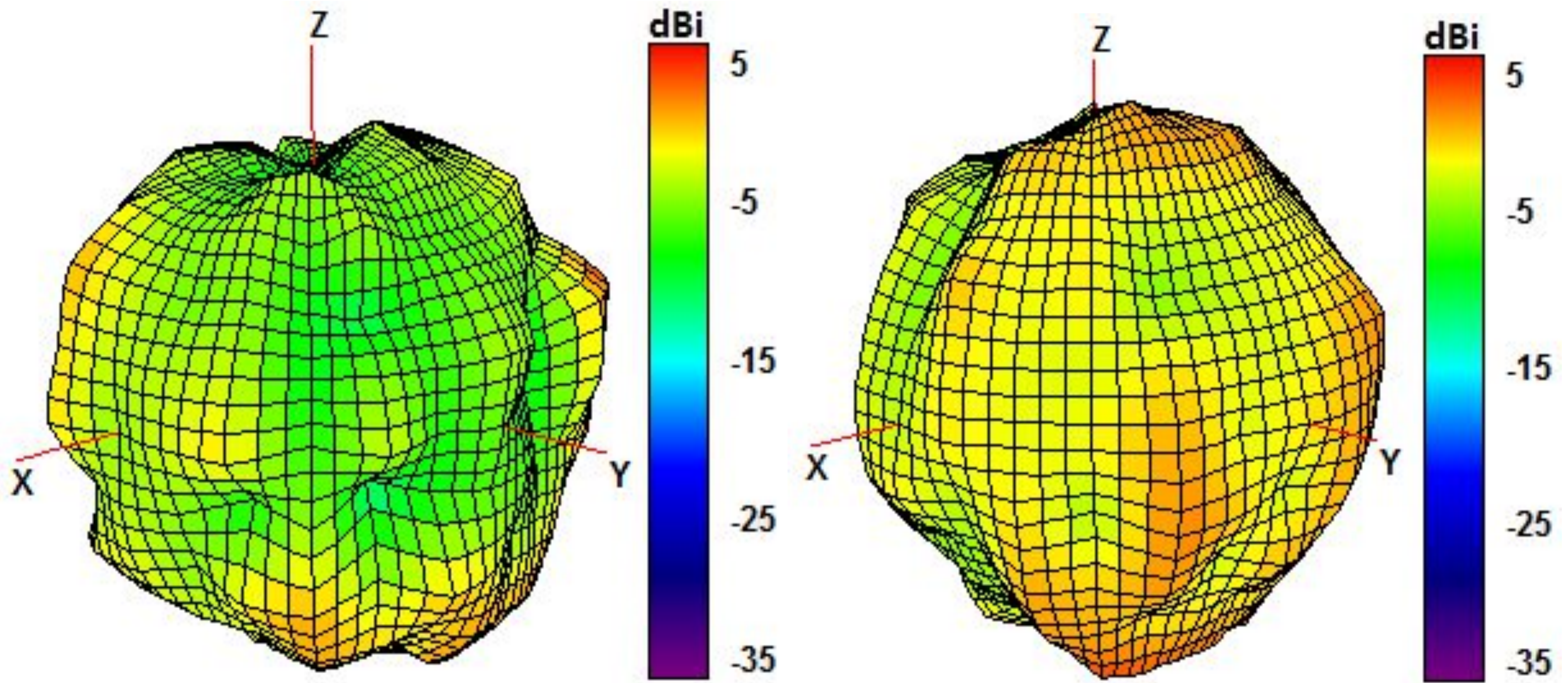
2100 and 2600 MHz Radiation pattern
