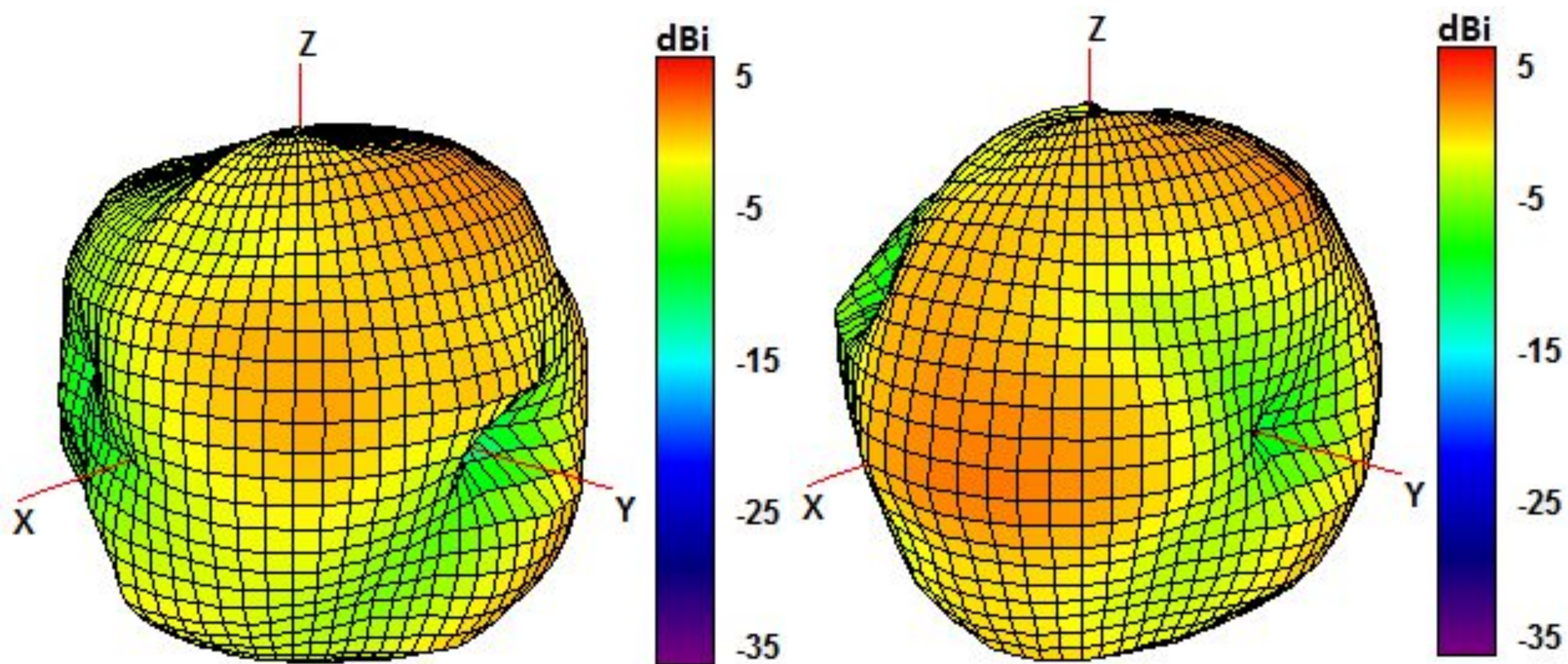
Cable 1: CELLULAR/LTE
