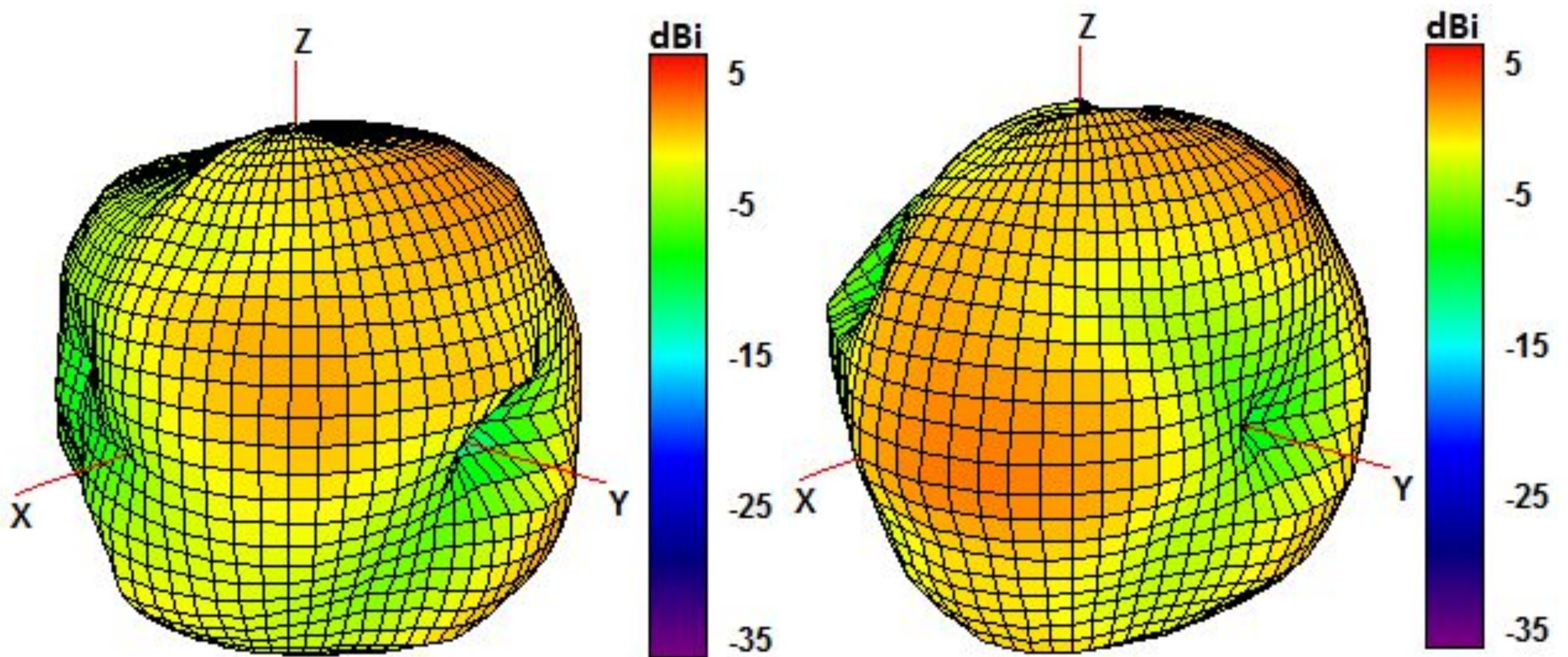
Cable 1: CELLULAR/LTE
