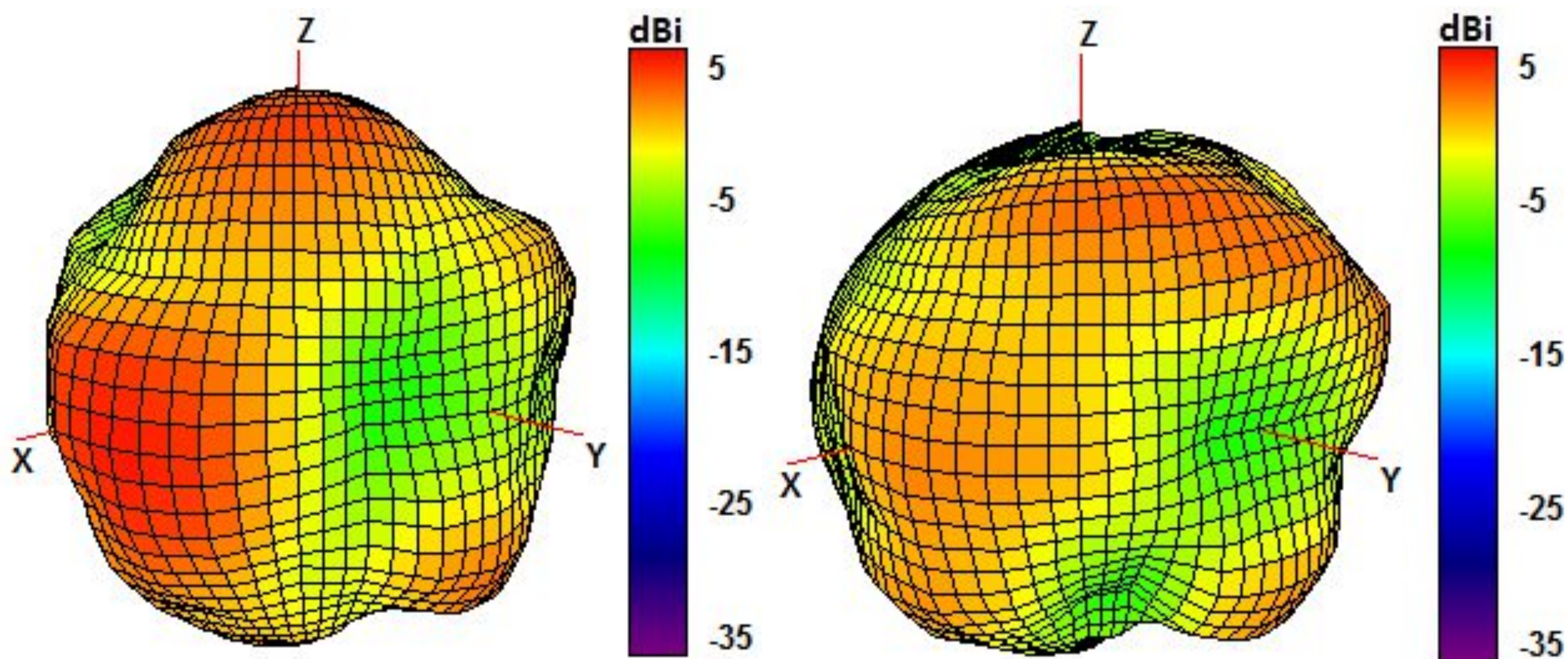
Cable 2: CELLULAR/LTE
