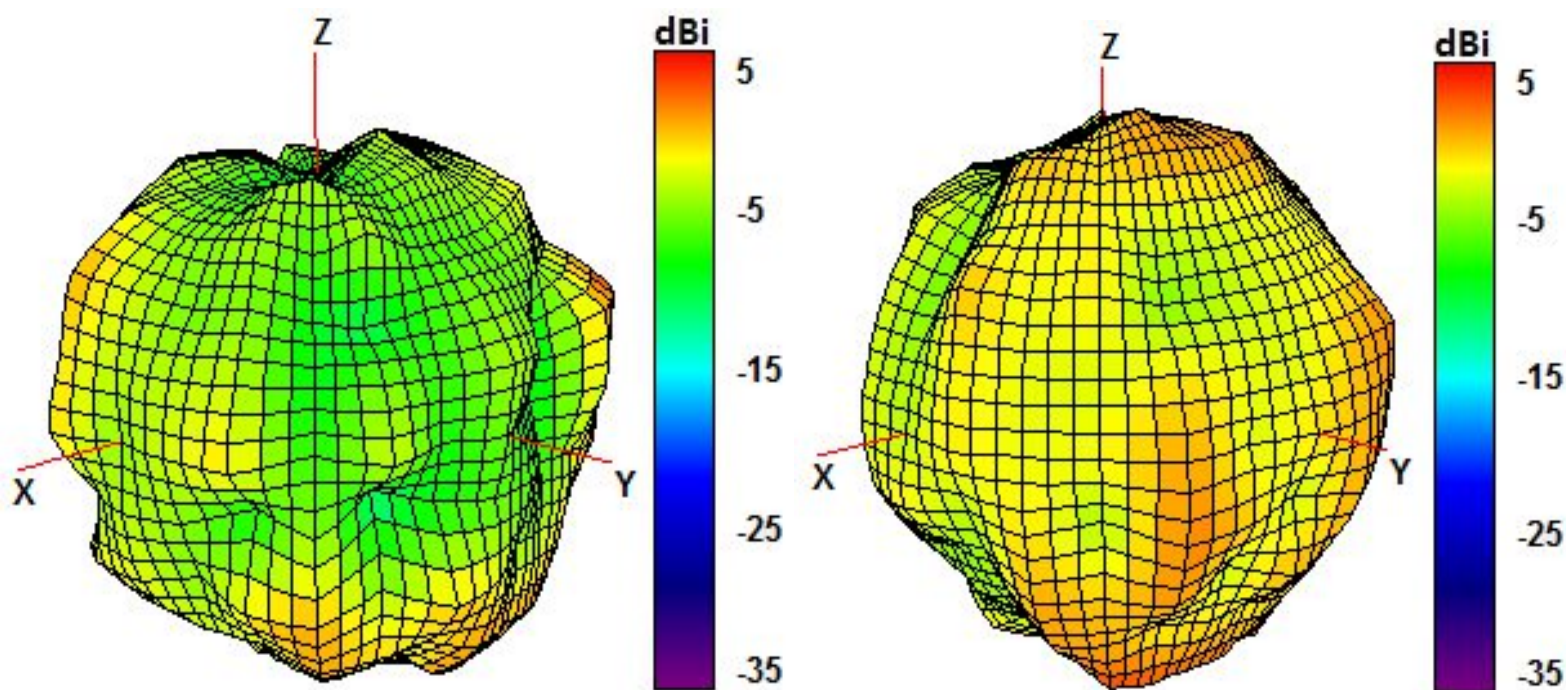
2100 and 2600 MHz Radiation pattern
