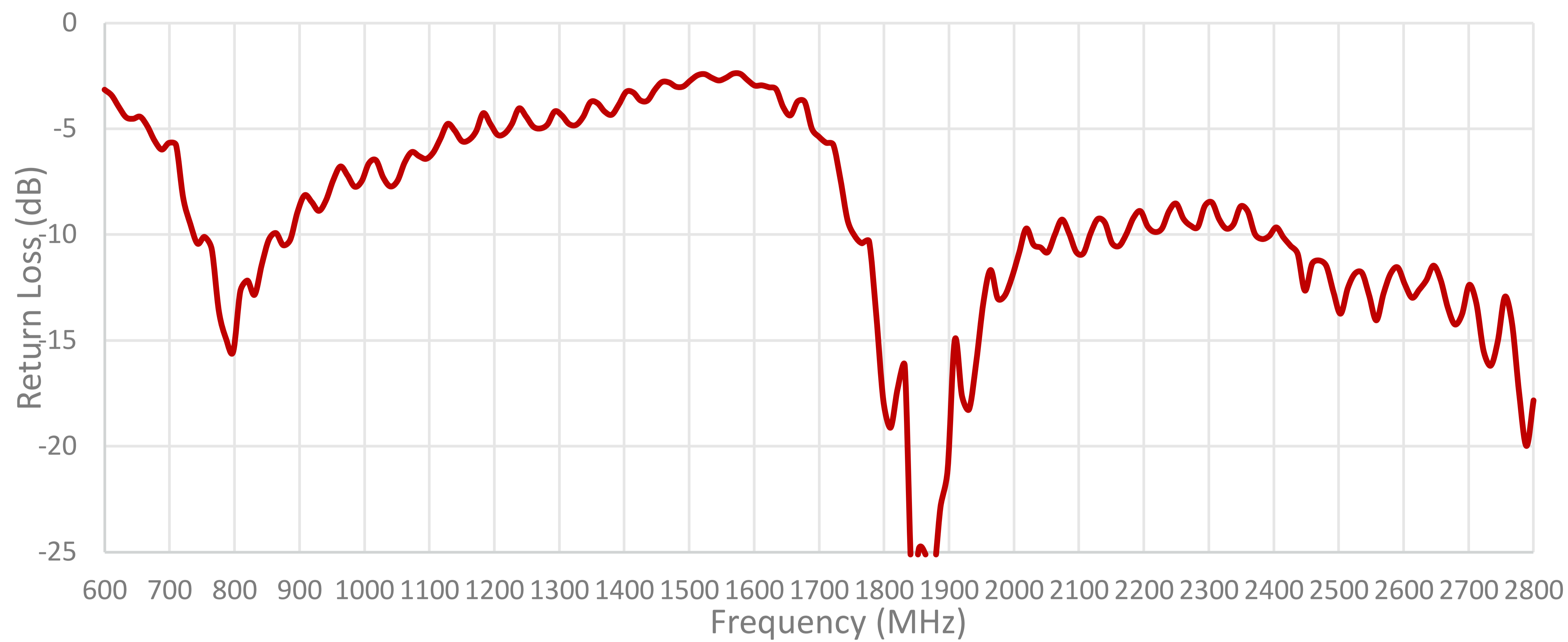
Cable 2: CELLULAR/LTE
