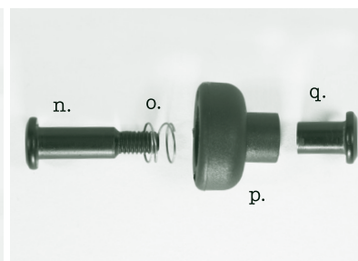
Schuifknop-set
