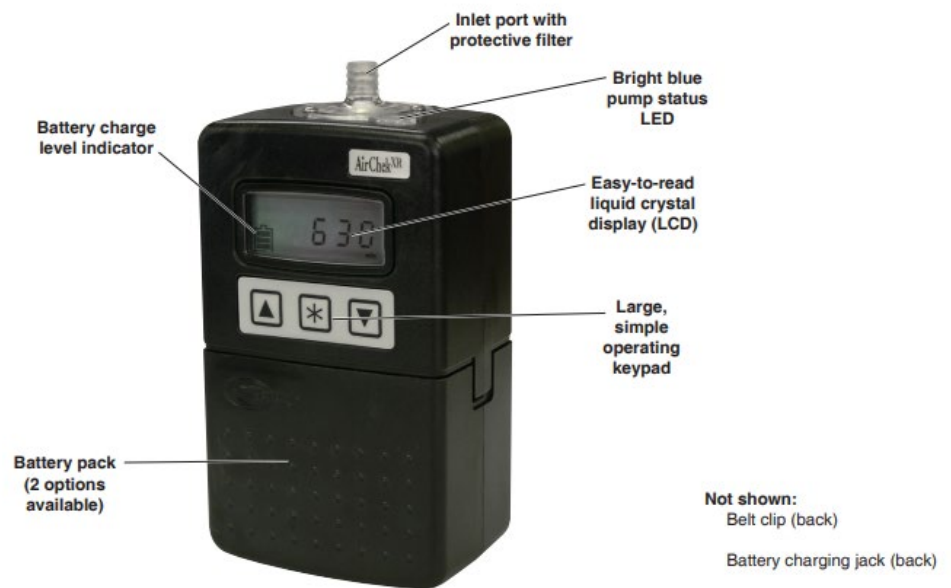
Figure 1. AirChek XR5000 Air Sample Pump
