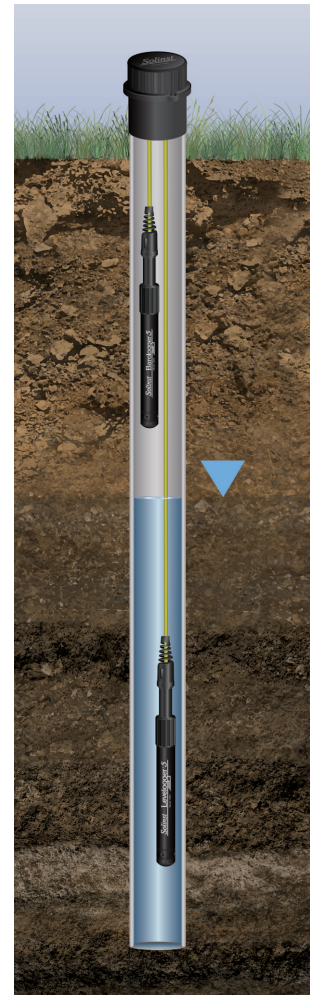
Barologger 5 and Levellogger 5 installed in Well Using L5 Direct Read Cables
