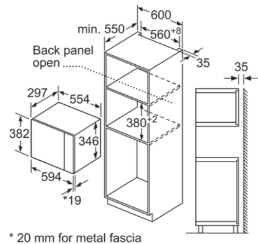
Built-in installation for model: M1
