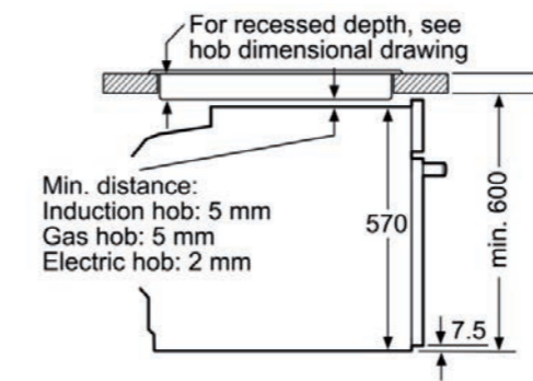
Built-in installation for models: B3 with a hob
