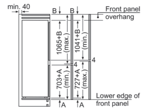
Built-in installation for model: M1
