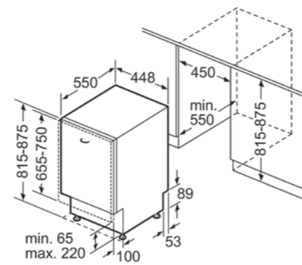
Built-in installation for model: D2
