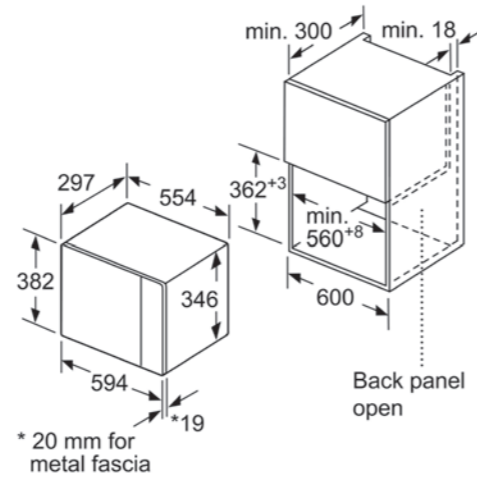
Built-in installation for model: M1
