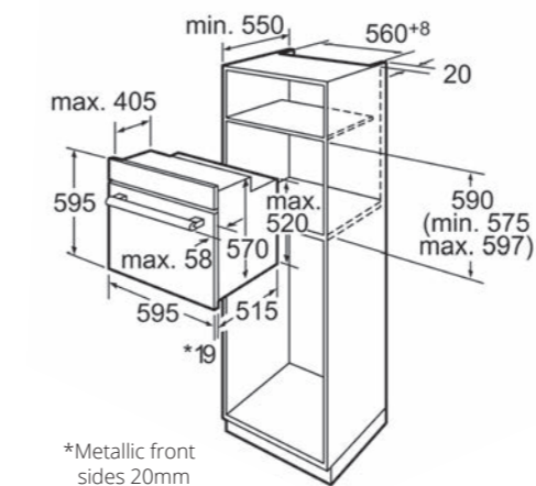
Built-in installation for models: B1, B2
