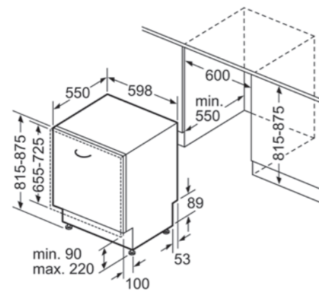
Built-in installation for model: D1
