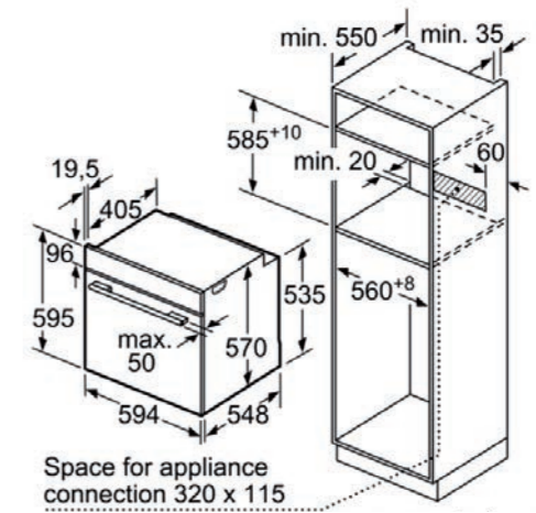
Built-in installation for models: B3
