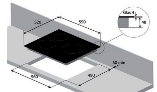
Built-in installation for models: H1, H2
