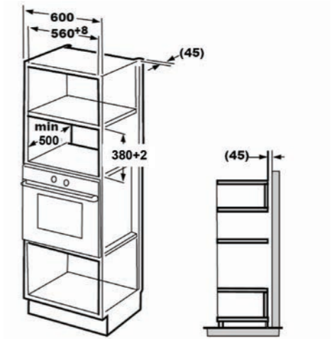
Built-in installation for model: M5
