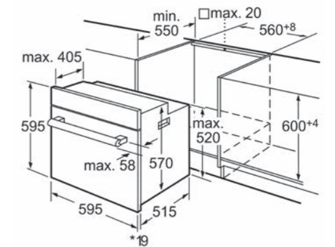
Built-in installation for models: B1, B2
