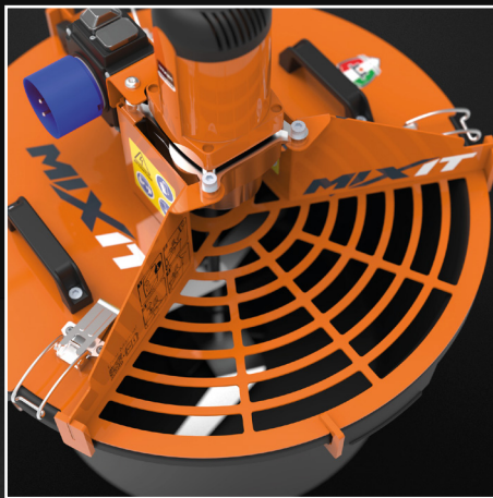
Material should be poured directly on the steel cover for the correct mixing.
