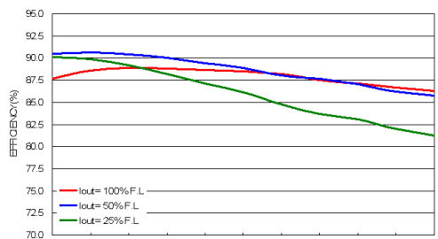
WAF(D)150-48S24W Efficiency vs. Input Voltage
