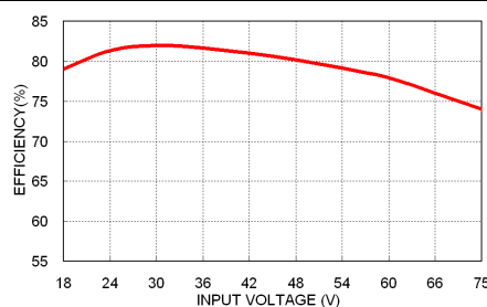
PDS03-48S05W Efficiency vs. Input Voltage
