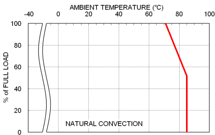
PDS03-48S05W Derating Curve
