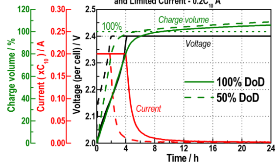
Charge with Constant Voltage - 2.40 V per cell at 20°C and Limited Current - 0.2C 10 A
