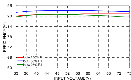
HAE200-48S05 Efficiency vs. Input Voltage
