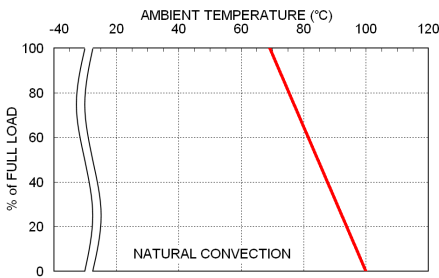
FKC08-48S05 Derating Curve
