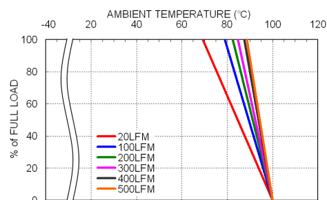
FEC15-48S05 Derating Curve With Heat-sink
