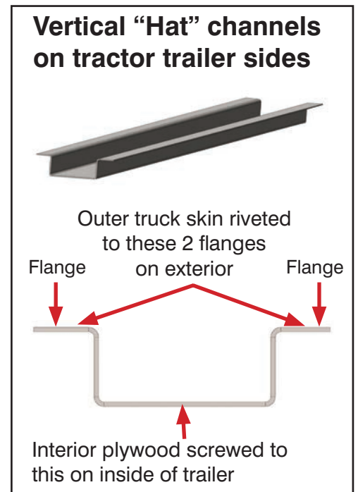
The outer alum or steel "skin" is riveted to "Hat" channels inside trailer.
