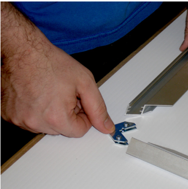
Step 4: Place Hardware Corners into Ends of Mitered Frame Rails
