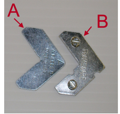
Step 3: Slide in Hardware Corners. Place (B) Plate (With Screws) Over (A) Plate.
