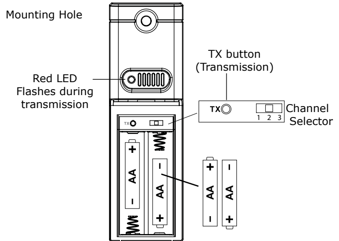
TX141TH-BCH Sensor
