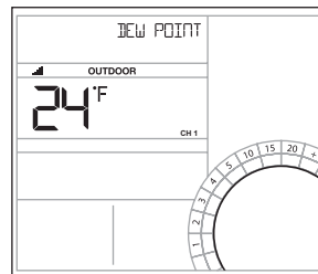
Dew Point
