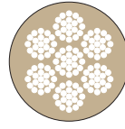
7 x 19 Construction
