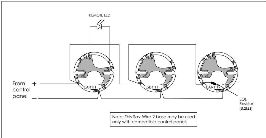
Sav-Wire base wiring diagram
