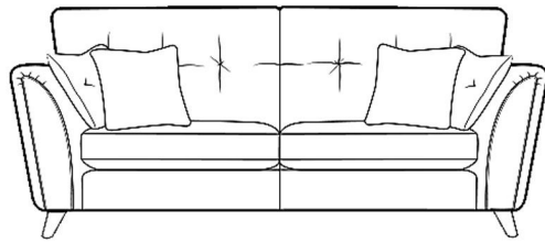
Grand sofa H 970mm W 2280mm D 1000mm
