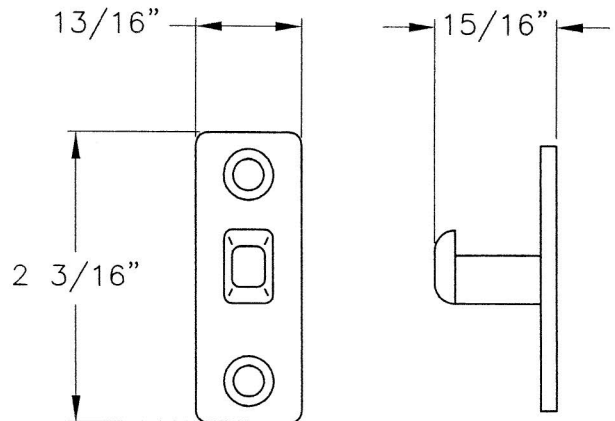
STRIKE FOR #558 MECHANISM PART # OT8066-8
