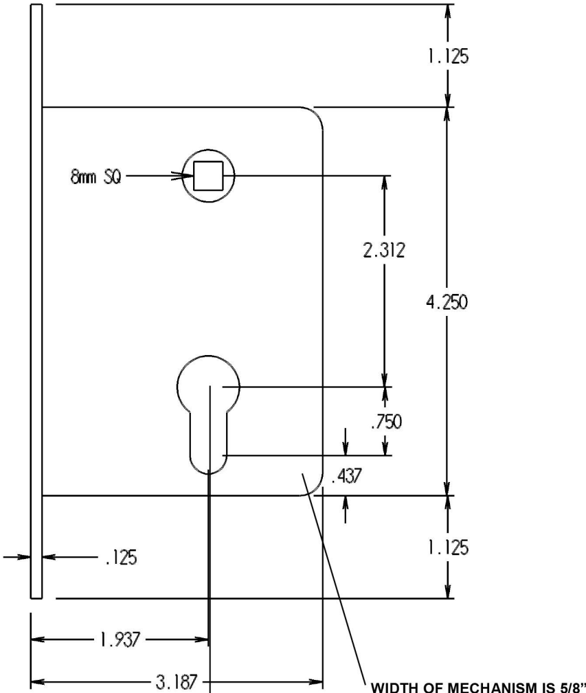
STRIKE FOR #558 MECHANISM PART # OT8066-8
