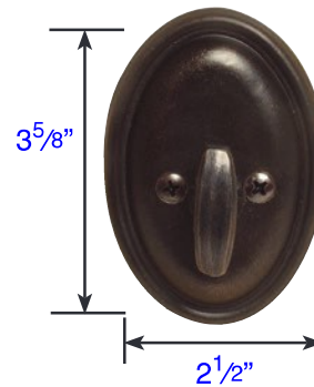
Interior Trim (8473) • Projection is 1 1/4" • Thickness is 9/16"
