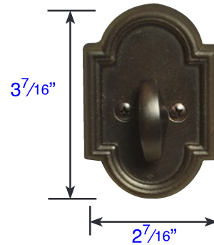
Interior Trim (8472) • Projection is 1 1/4" • Thickness is 9/16"
