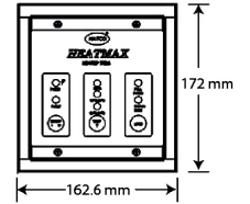
Control Box
