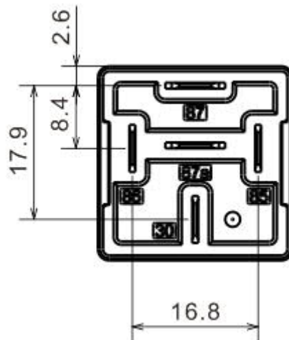
(底视 Bottom View)
