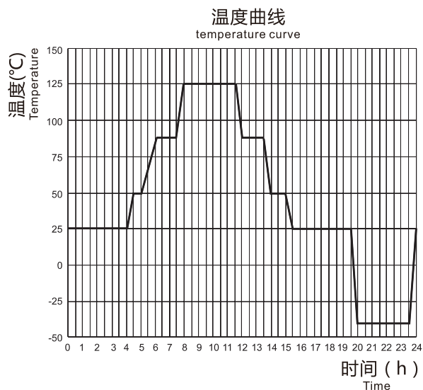
3. 电耐久试验环境温度曲线 Environmental Temperature Curve Of Electric Endurance Test
