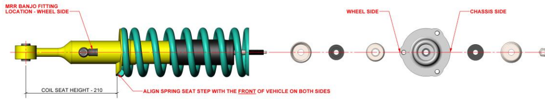
TOYOTA LANDCRUISER (PRADO 120) / 4RUNNER (GEN 4) RIGHT HAND STRUT SHOWN
