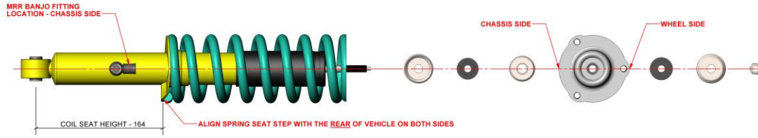
TOYOTA LANDCRUISER (PRADO 90) RIGHT HAND STRUT SHOWN
