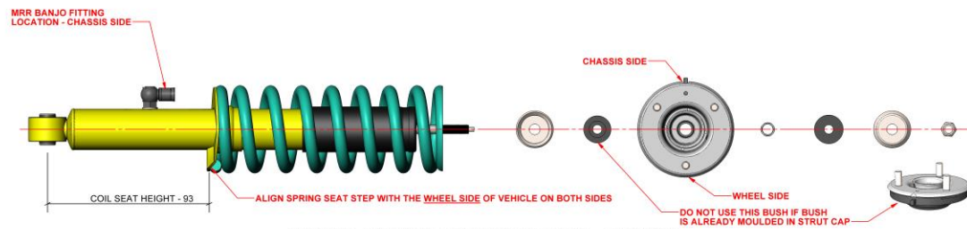
NISSAN NAVARA / FRONTIER (D40 - STX500) LEFT HAND STRUT SHOWN
