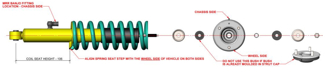
NISSAN NAVARA / FRONTIER (D40/D23 NP300) LEFT HAND STRUT SHOWN
