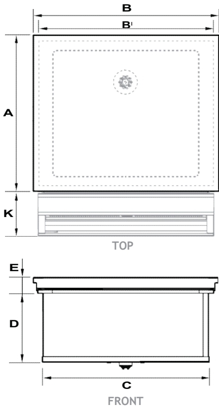
Cabinetry dimensions inches (mm)
