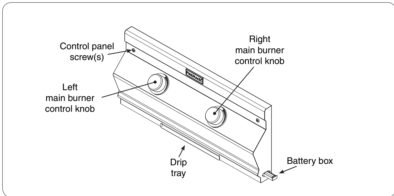
Fig. 23-1 C430s controls
