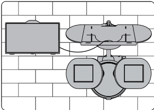
6. Use the additionally provided accessories and repeat steps 1 to 4 for installing the detached solar panel in an optimal position.
