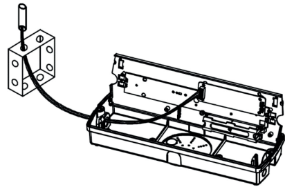
3. Electrical Connections. Make the proper supply wire connections. Connect L and N to building utility. If using maintained working mode, keep L and SL jumper connected. If using the non-maintained working mode, disconnect L and SL and dispose of the jumper.
