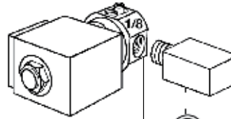
560066/22=220/50/60V 560066/11=110/60V
