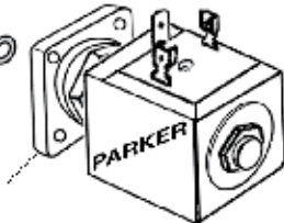
634294/22 =220/50/60V 634294/11 =110/60V
