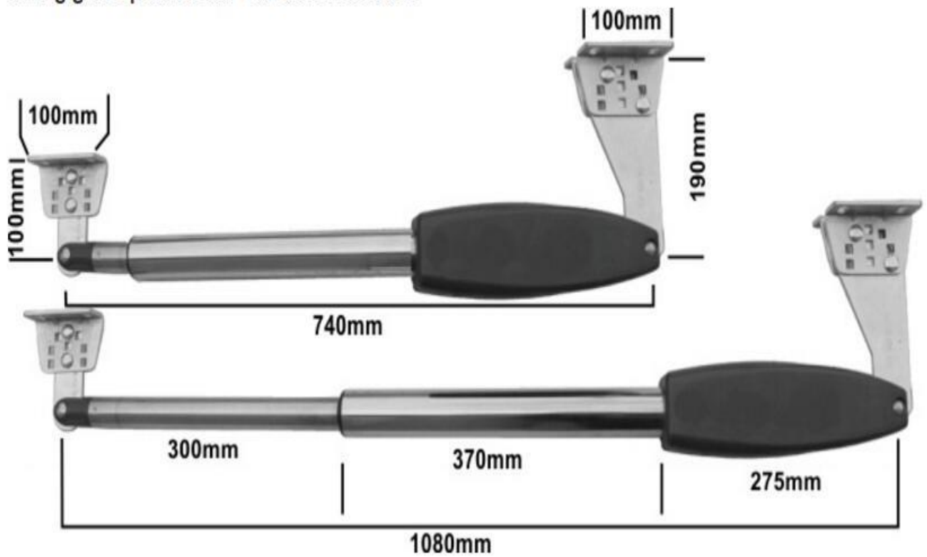
Swing gate opener PKM C02 dimension size
