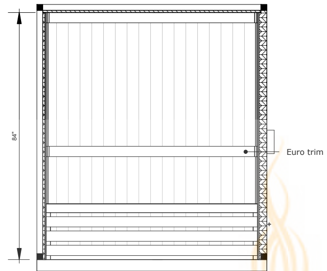
B Inside Elevation View 2 3/8" = 1'-0"
