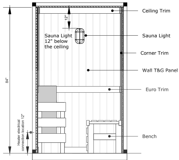
A Inside Elevation View 1 3/8" = 1'-0"
