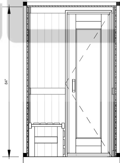
C Inside Elevation View 3 3/8" = 1'-0"
