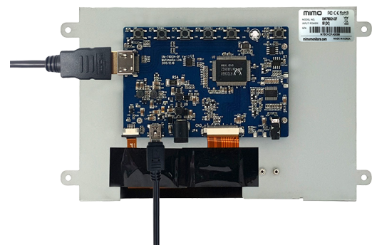
UM-760CH-OF Back view
