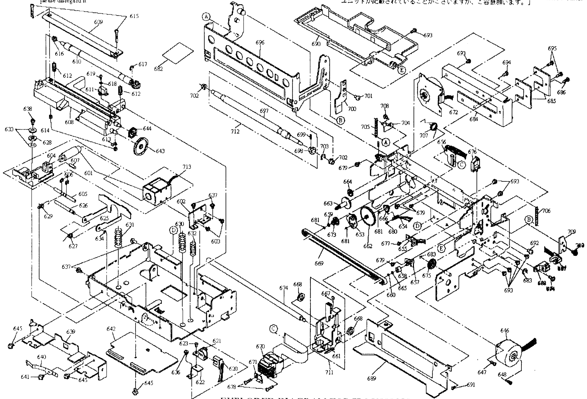
EXPLODED DIAGRAM FOR TM-U590 NO.2
