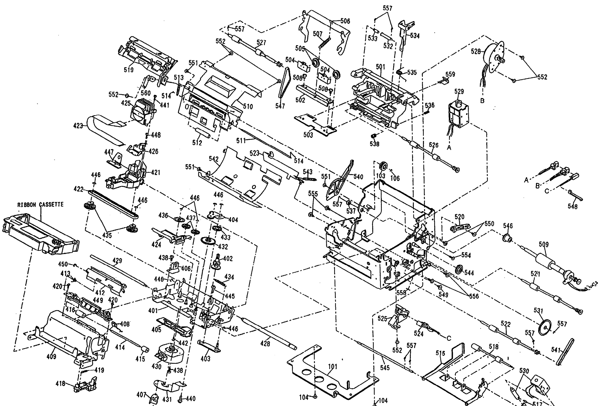
EXPLODED DIAGRAM FOR TM-U375 NO. 2
