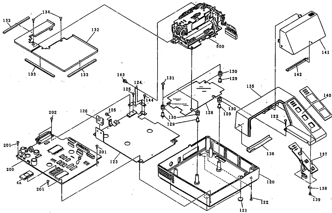
EXPLODED DIAGRAM FOR TM-290 (1)
