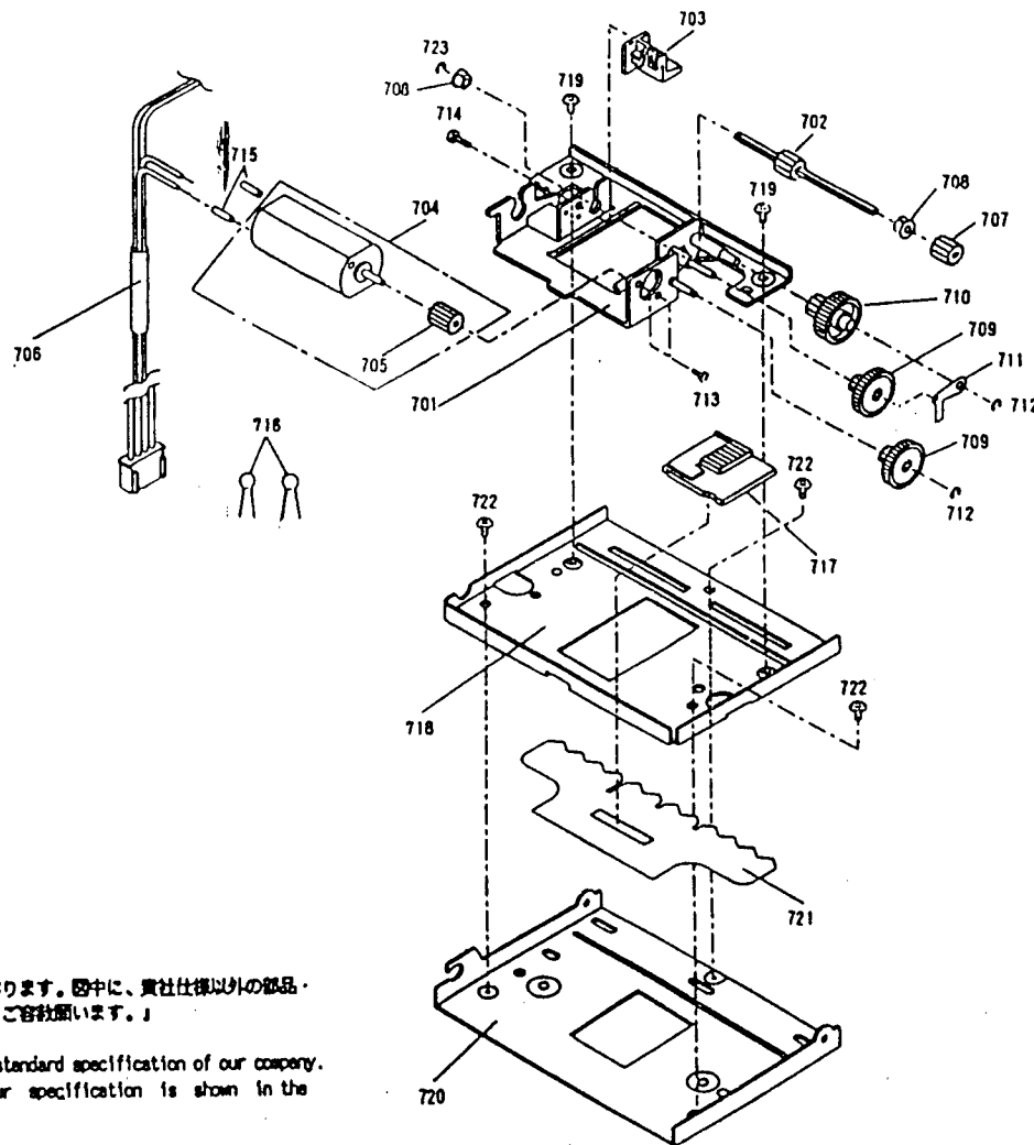
EXPLODED DIAGRAM FOR TM-300A/B (AUTO CUTTER UNIT)
