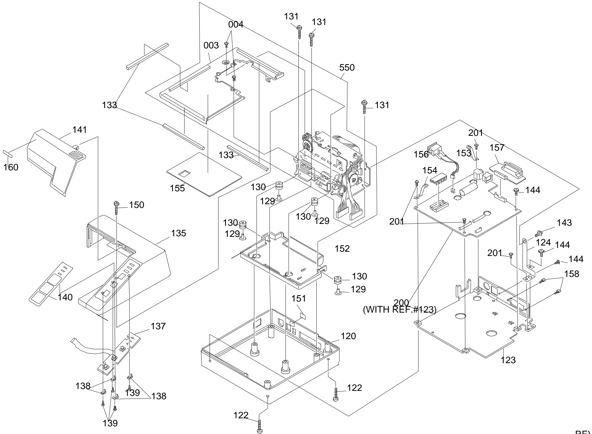
EXPLODED DIAGRAM FOR TM-U295 NO.1
