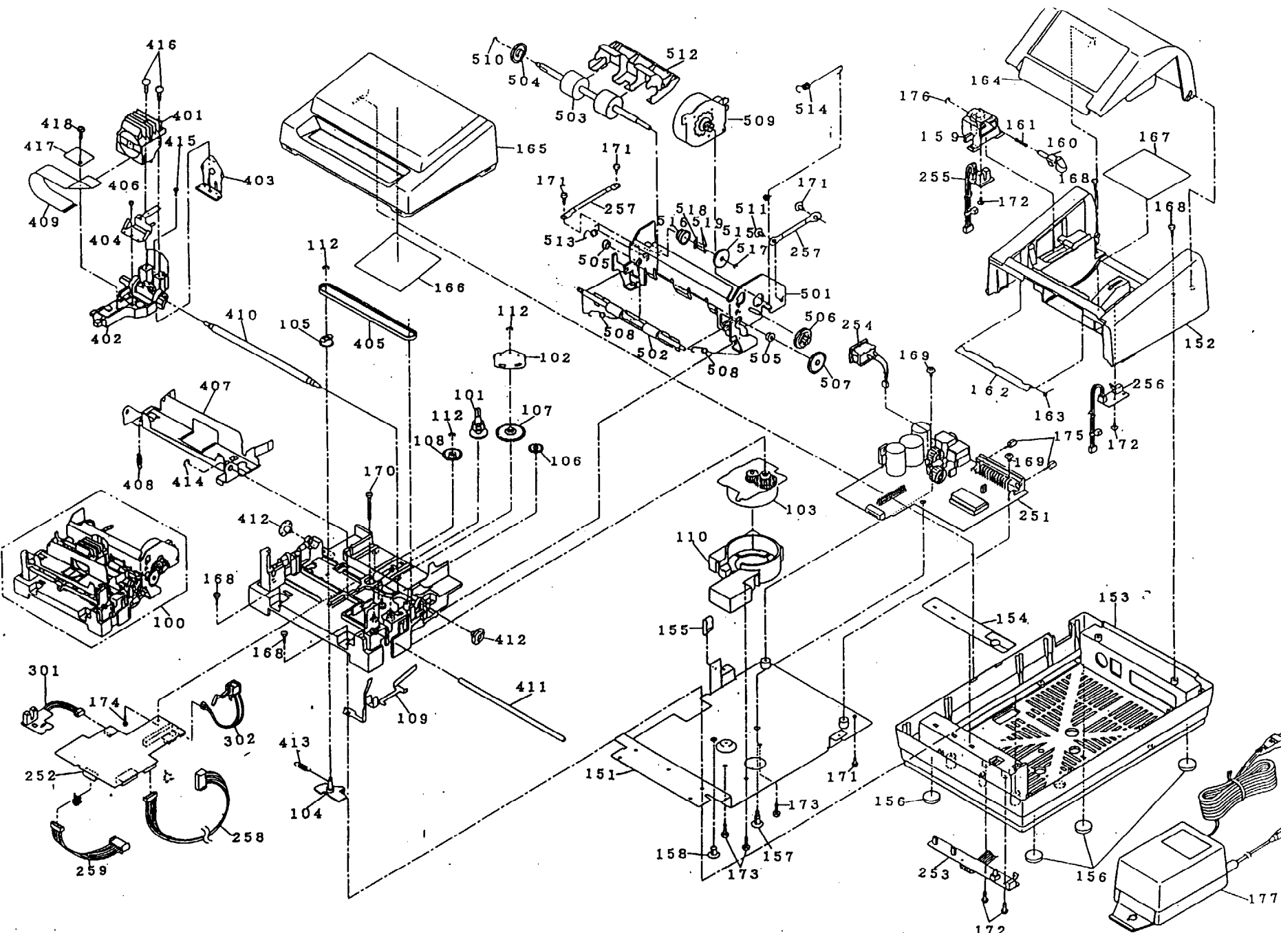
EXPLODED DIAGRAM FOR TM-300D
