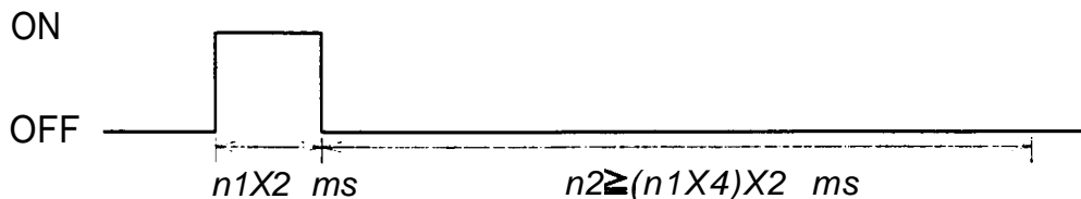
Figure D-1 . Drawer Drive Signal Waveform
