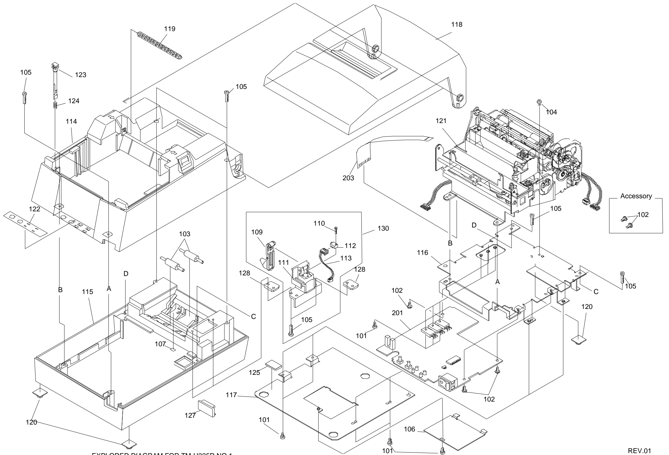
EXPLODED DIAGRAM FOR TM-U325D NO.1
