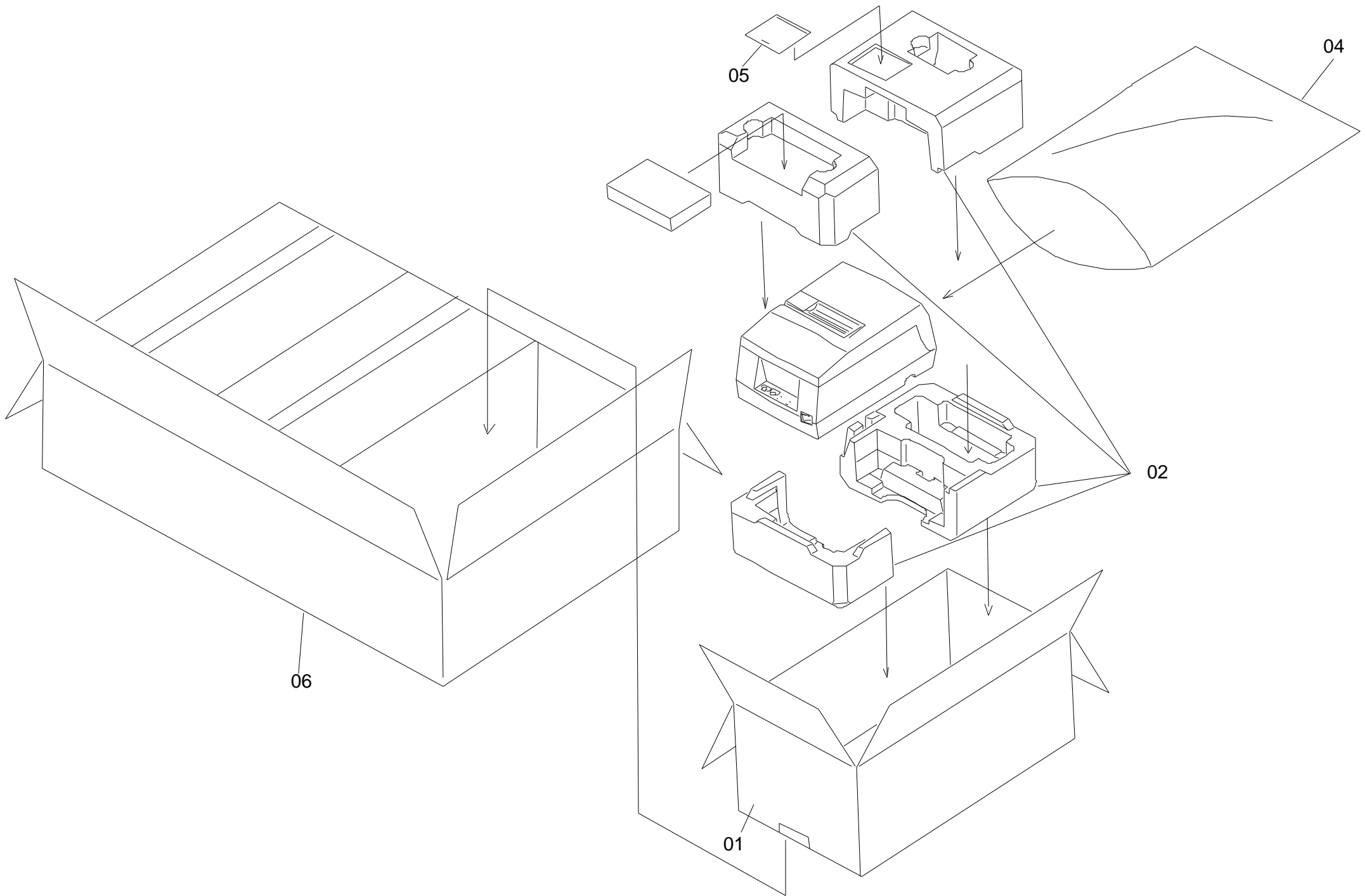
PACKING MATERIAL FOR TM-U325D/U325PD SEREIES
