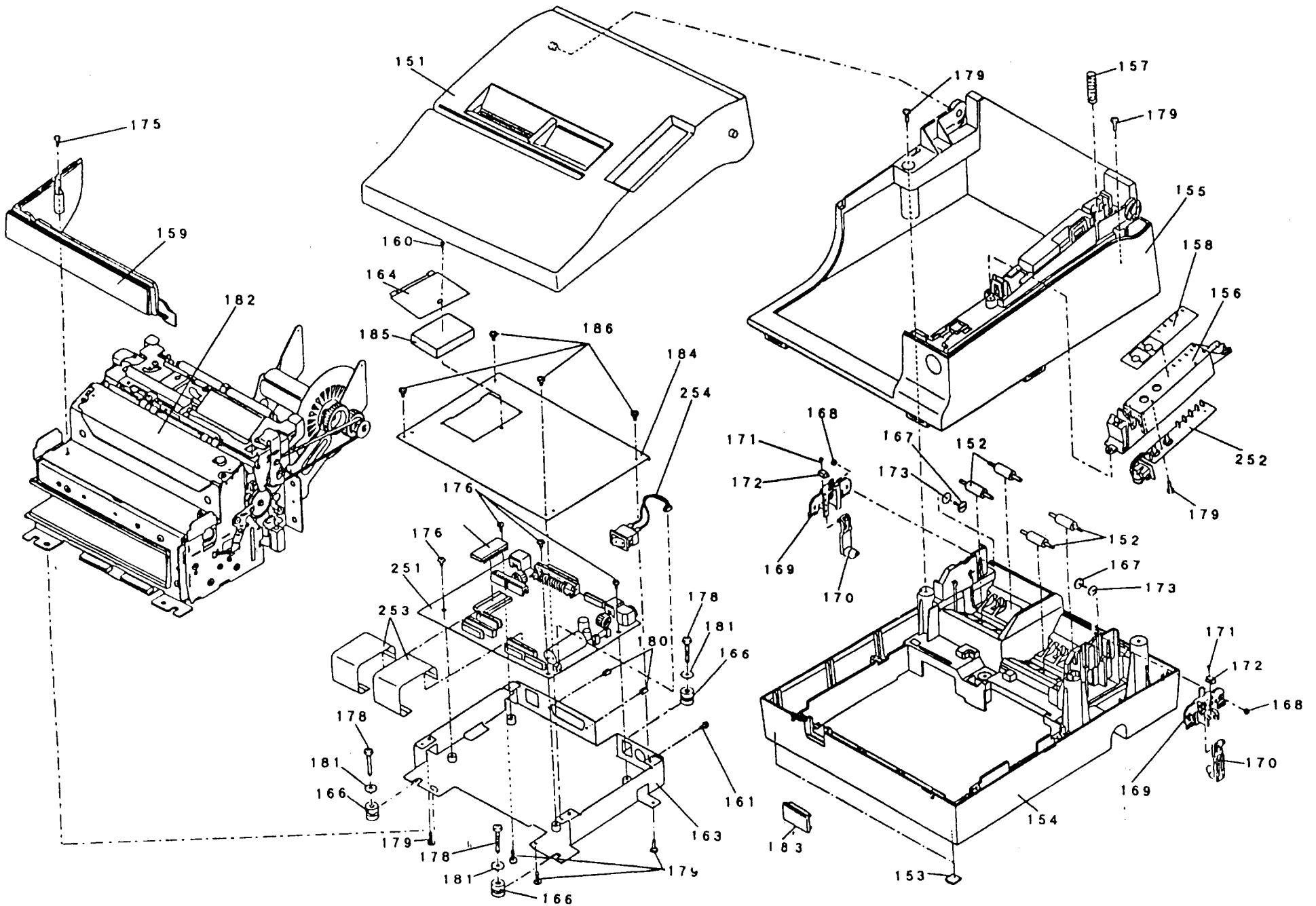
EXPLODED DIAGRAM FOR TM-U950 NO. 1
