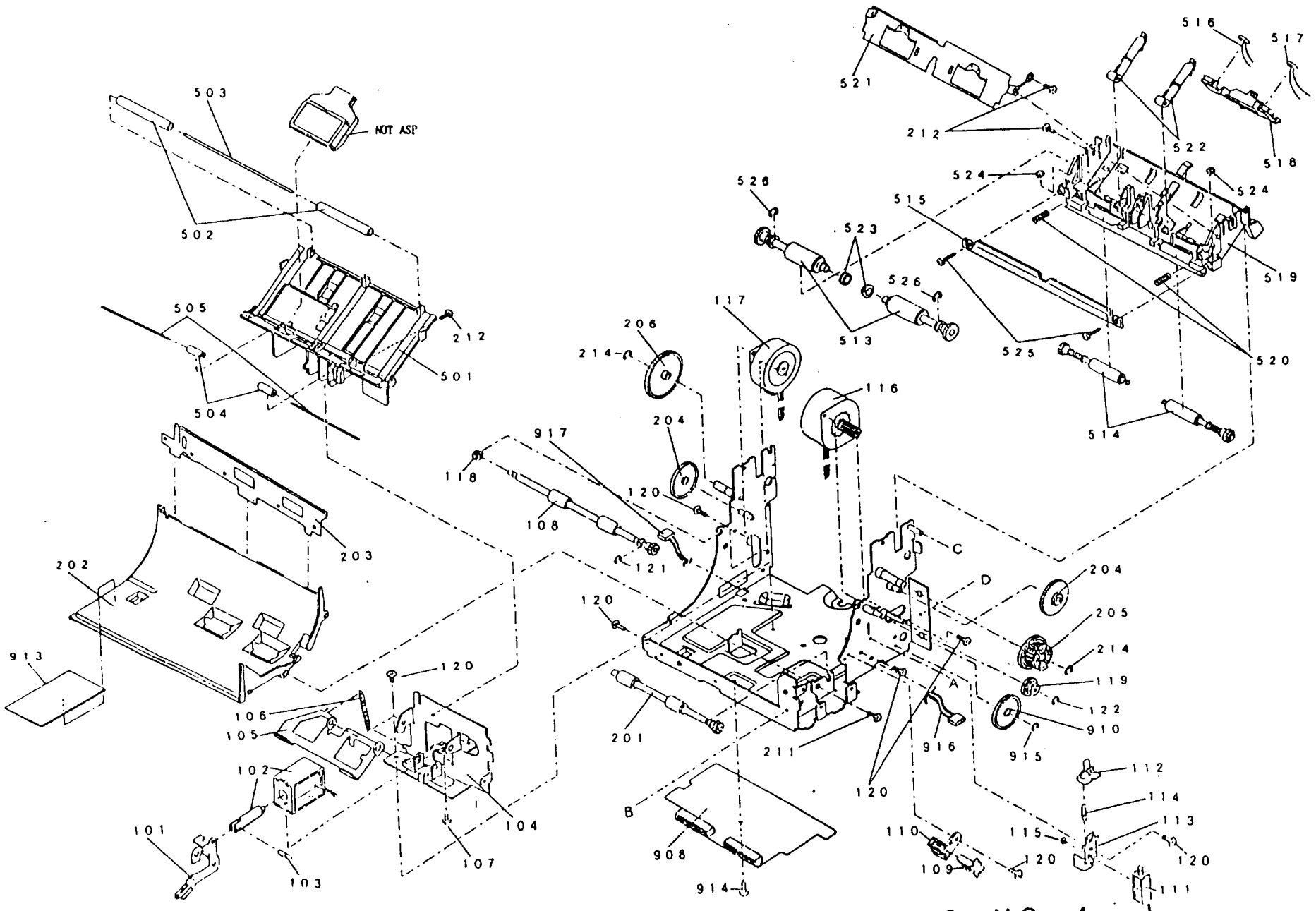
EXPLODED DIAGRAM FOR TM-U950 NO. 4
