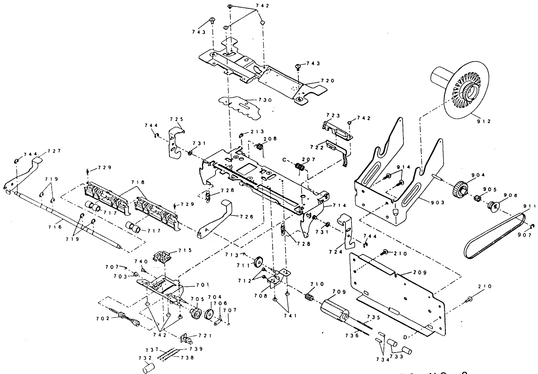
EXPLODED DIAGRAM FOR TM-U950 NO. 3
